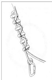
Six-Bar Rappel Rack
